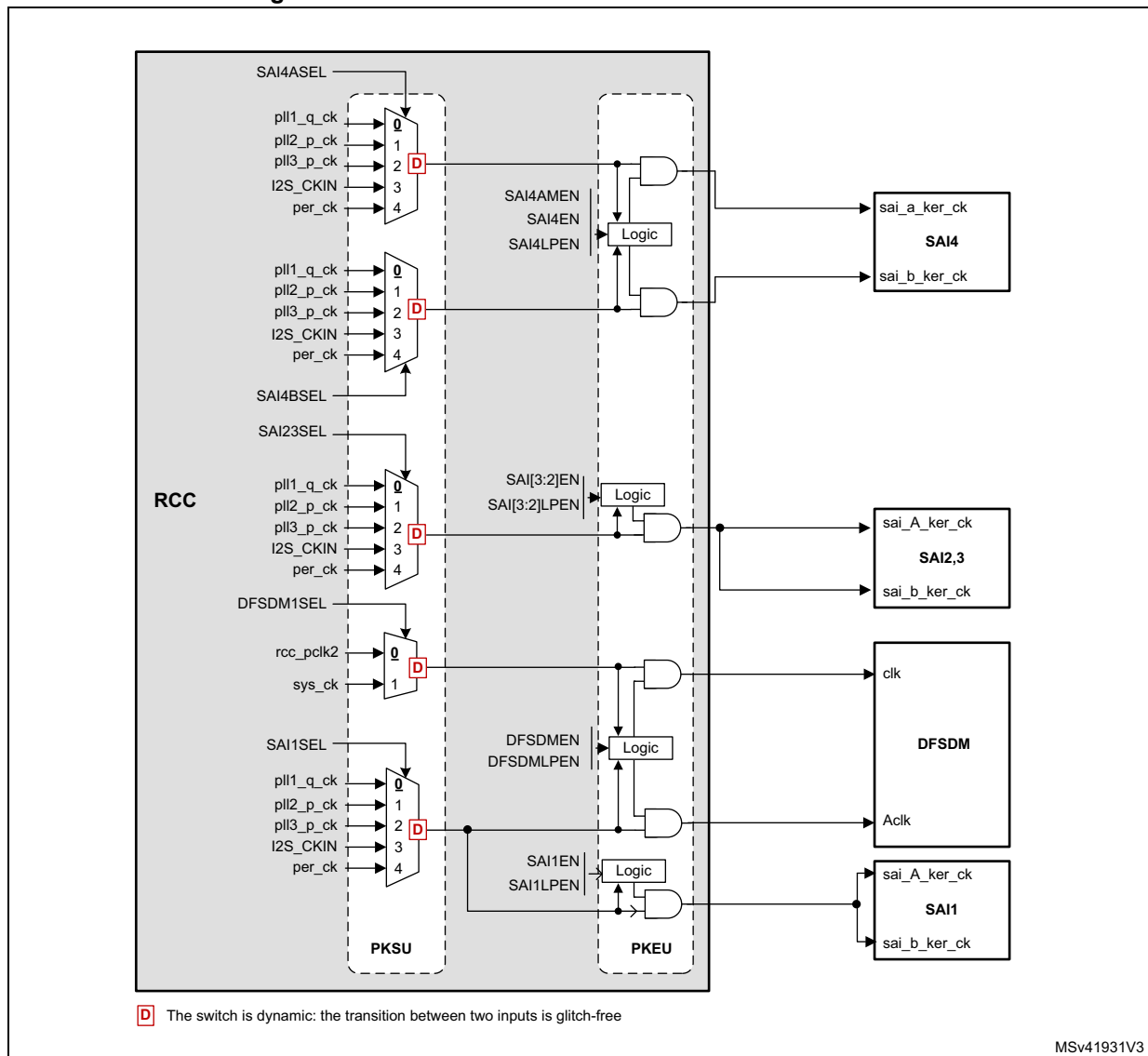
Figure 50. Kernel clock distribution for SAI4 and DFSDM
